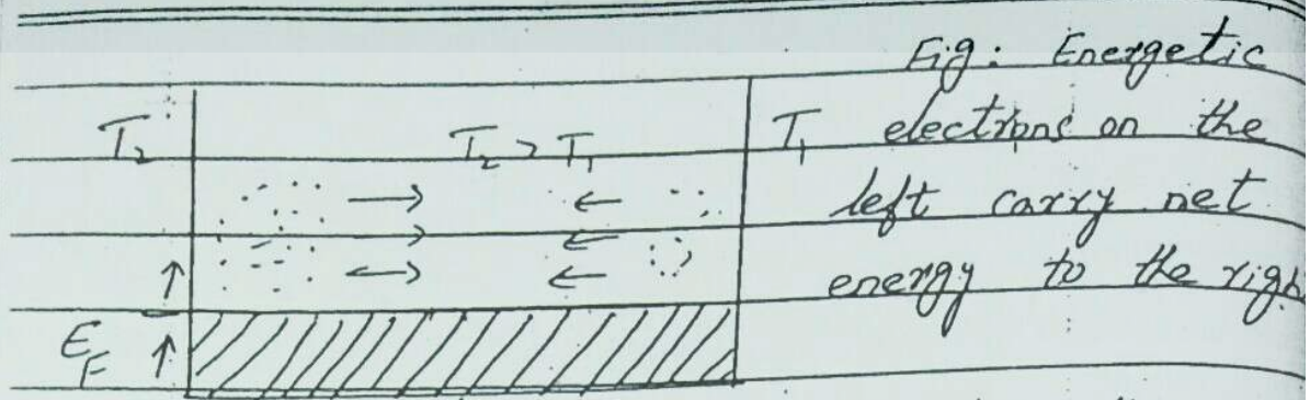
Figure:- The physical process for Thermal Conductivity.
